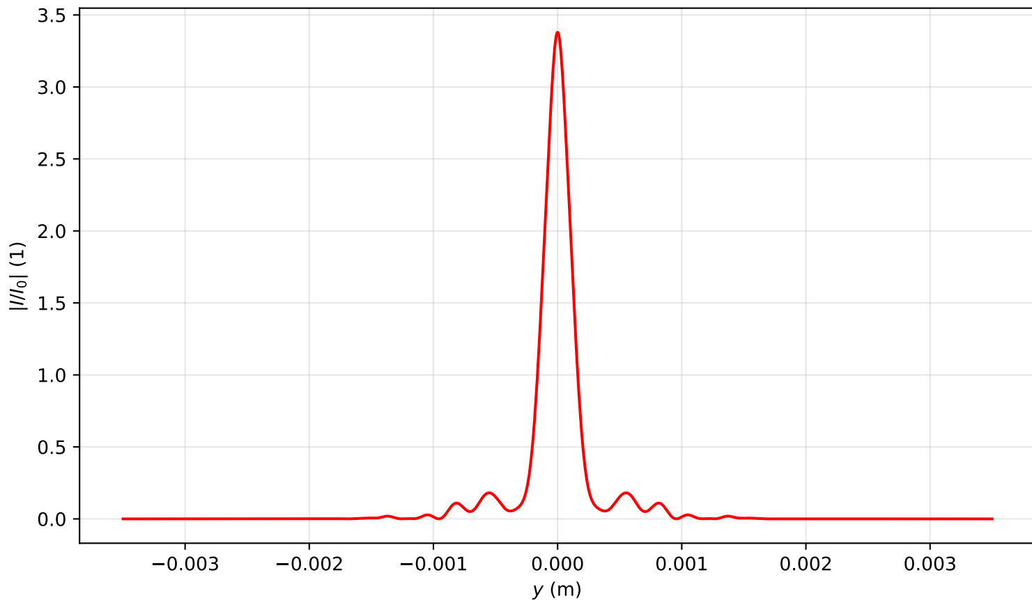
Intensity profile I(x=0, y, z=0.955)/I_0 , P_{in}=8.5P_{cr} , artificial time
